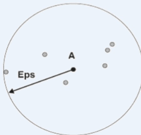
Figure 8.20. Center-based density.
